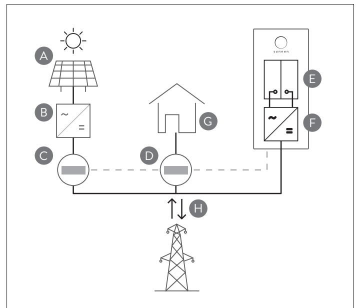
Fig. 4 Self-consumption mode
