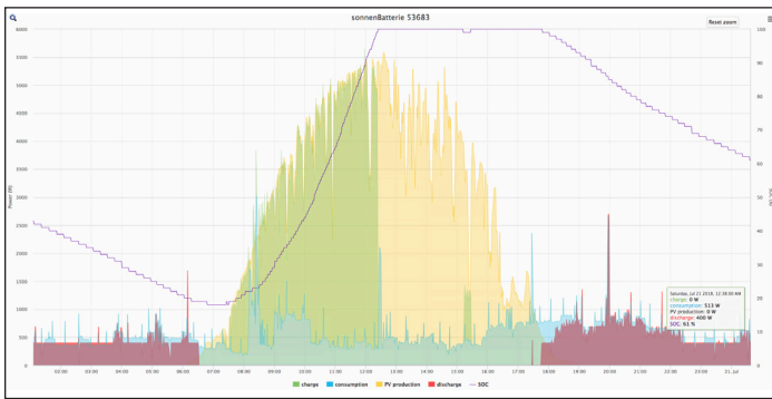
Fig. 13 History view
