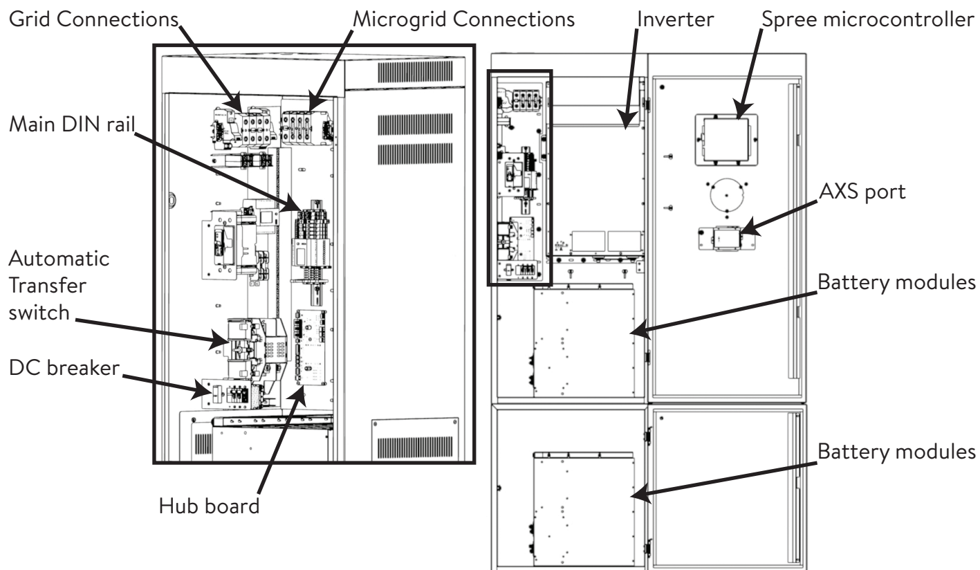
Fig. 2 ecoLinX 1.5 key components
