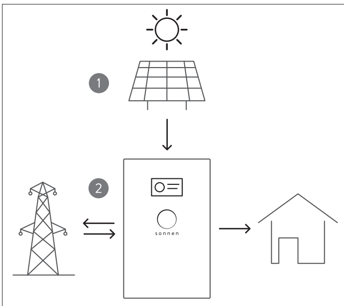
Fig. 3 Energy flow
